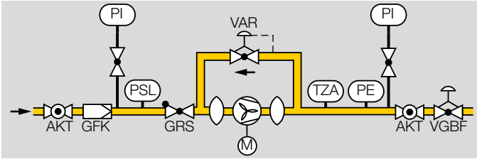
Gas pressure booster flowchart
